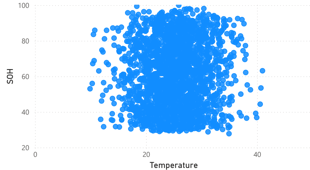
Temperature vs battery health (SOH)
