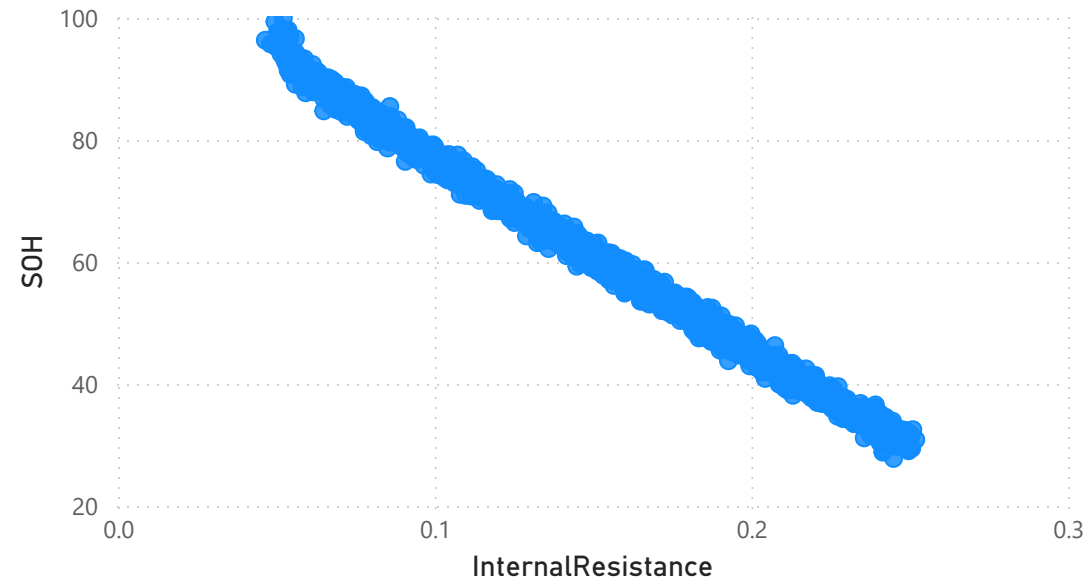
InternalResistance vs SOH
