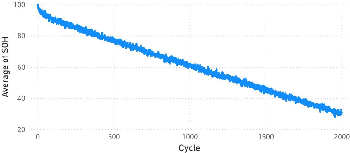
Battery Health Degradation Over Cycles
