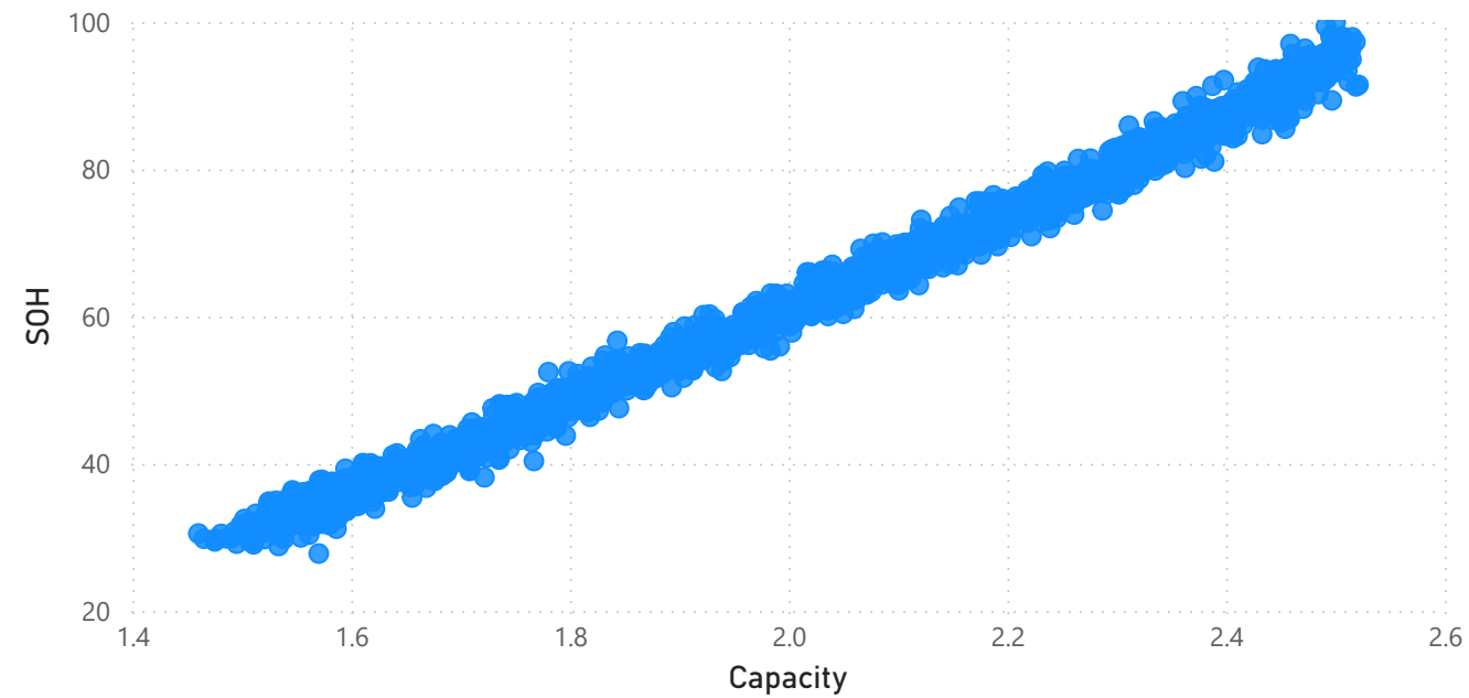
Capacity vs SOH
